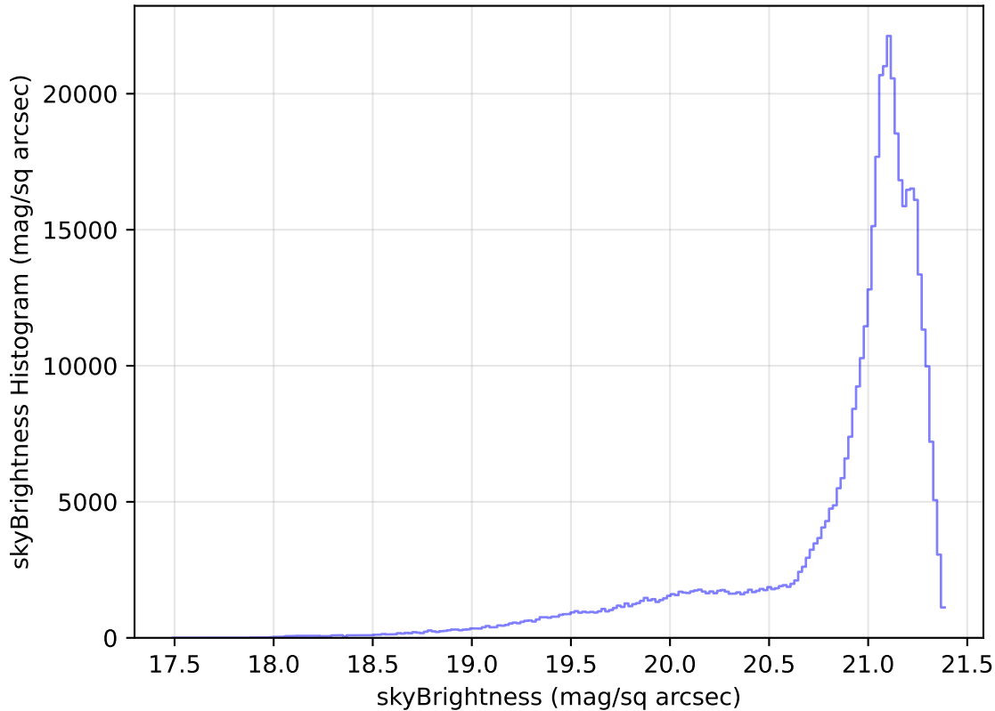
internal_u_expt30_nscale0.9v3.4_10yrs All sky r band: skyBrightness Histogram
