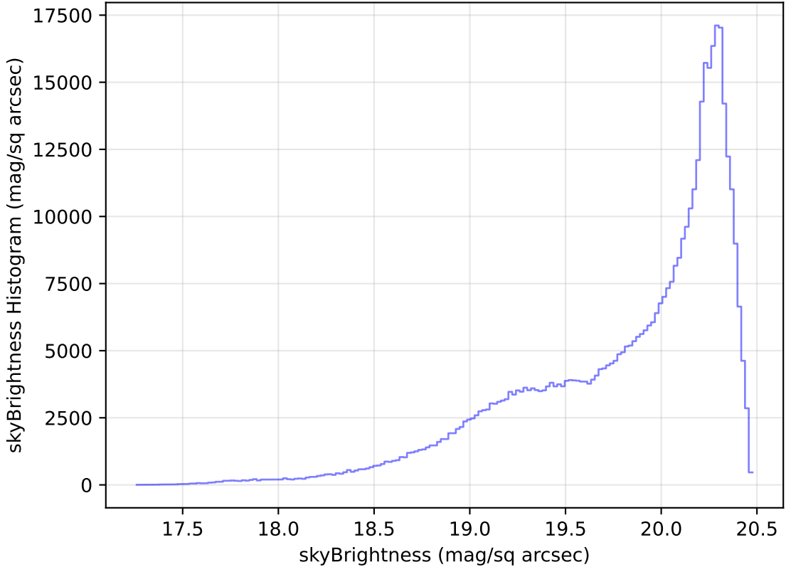
internal_u_expt30_nscale0.9v3.4_10yrs All sky i band: skyBrightness Histogram
