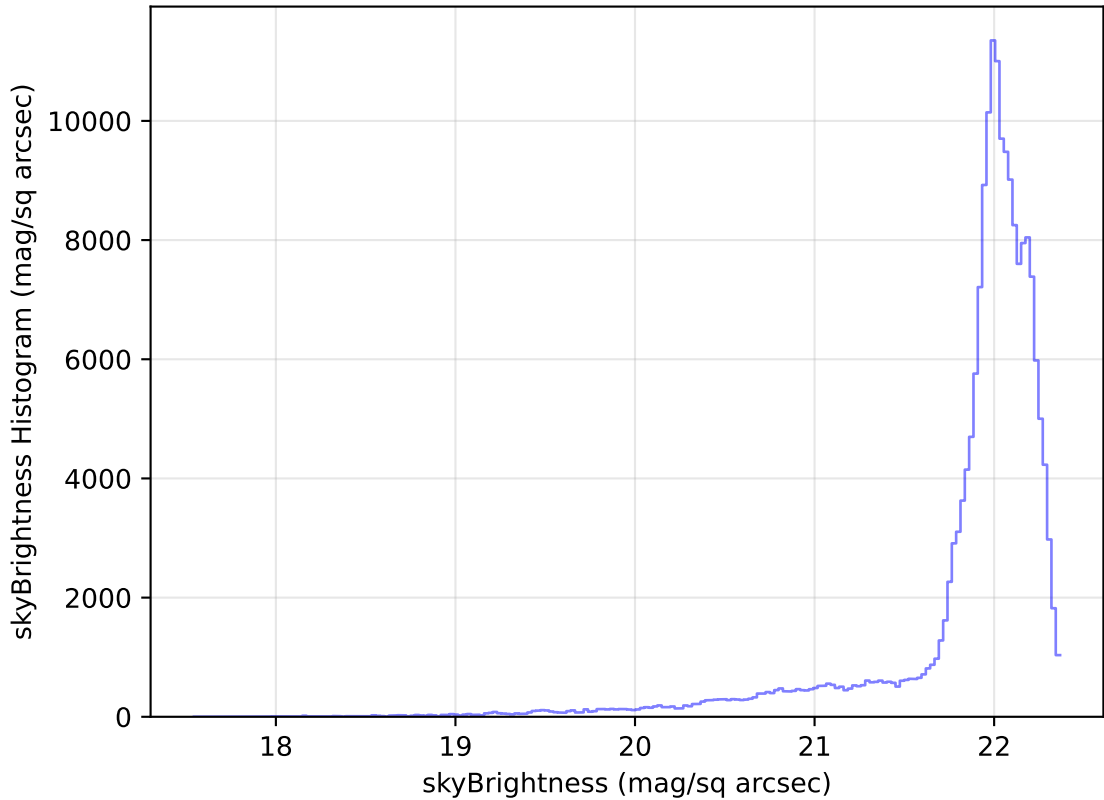
internal_u_expt30_nscale0.9v3.4_10yrs All sky g band: skyBrightness Histogram
