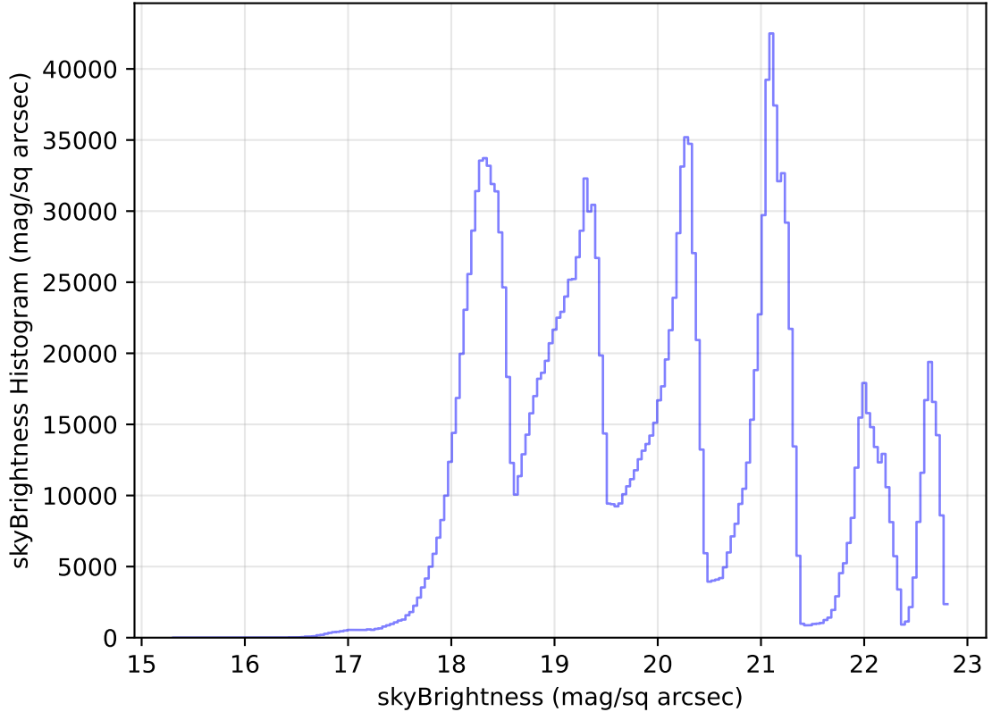
internal_u_expt30_nscale0.9v3.4_10yrs All sky all bands: skyBrightness Histogram
