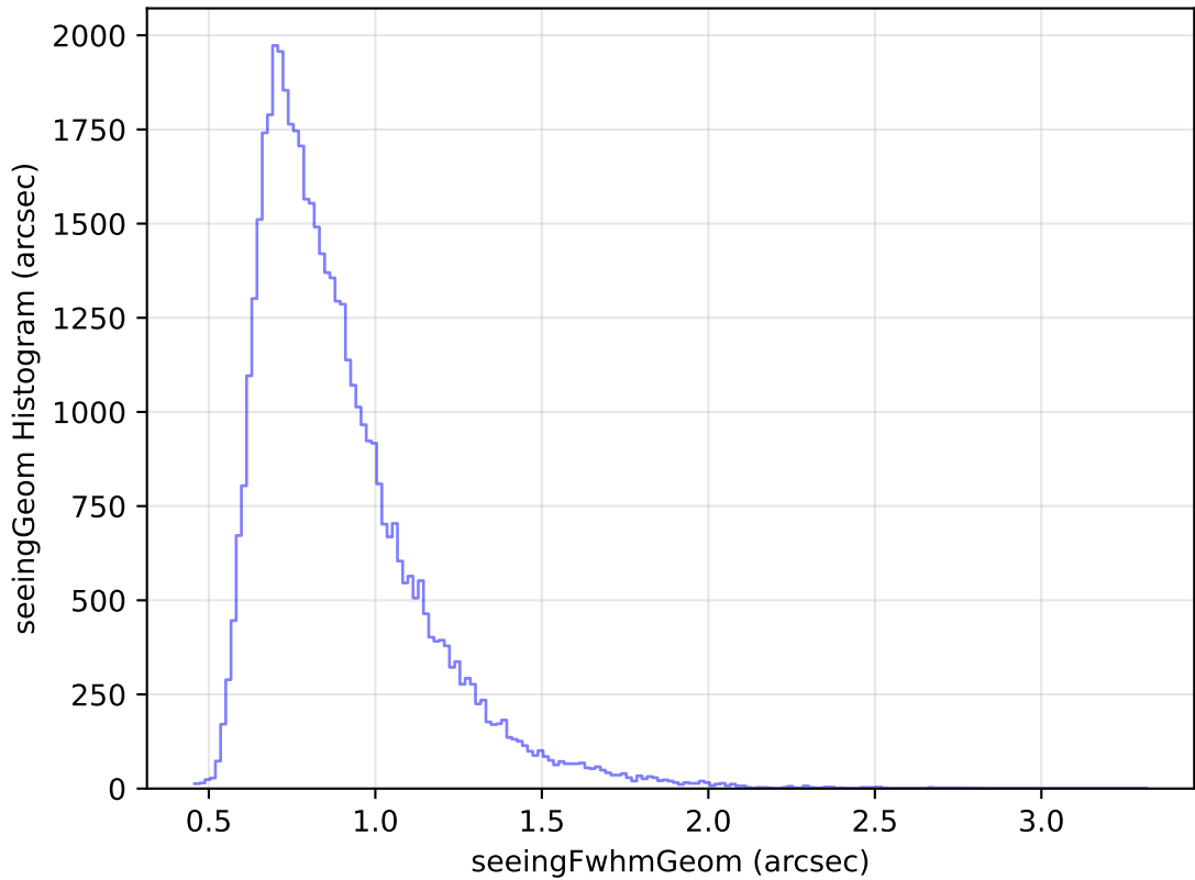
internal_u_expt30_nscale0.9v3.4_10yrs Yr 1 r band: seeingGeom Histogram
