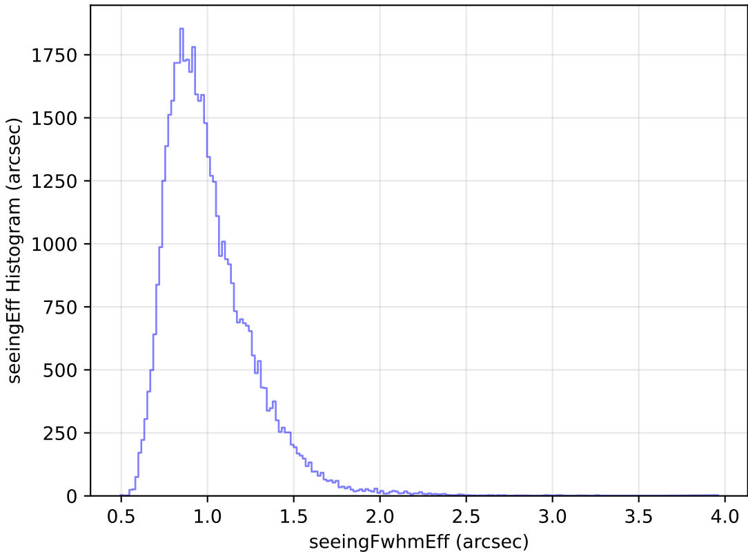
internal_u_expt30_nscale0.9v3.4_10yrs Yr 1 y band: seeingEff Histogram
