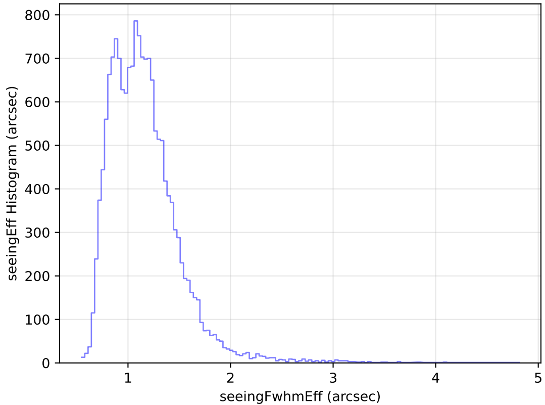
internal_u_expt30_nscale0.9v3.4_10yrs Yr 1 u band: seeingEff Histogram
