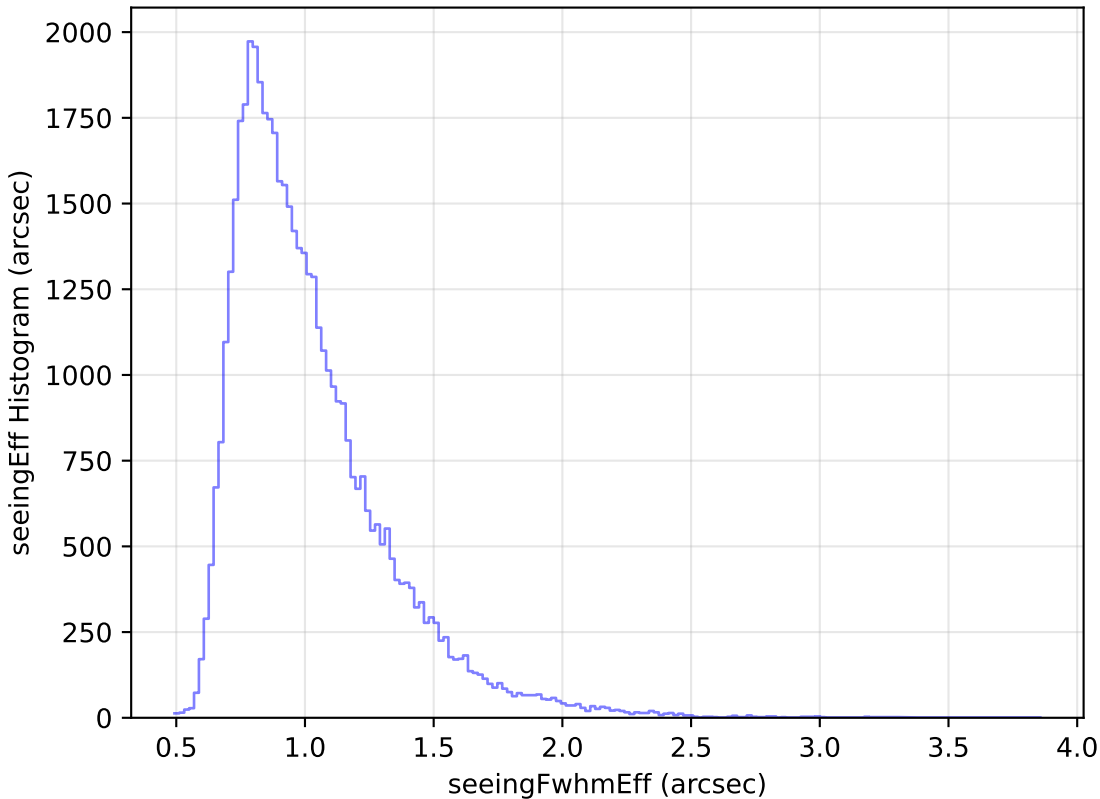
internal_u_expt30_nscale0.9v3.4_10yrs Yr 1 r band: seeingEff Histogram
