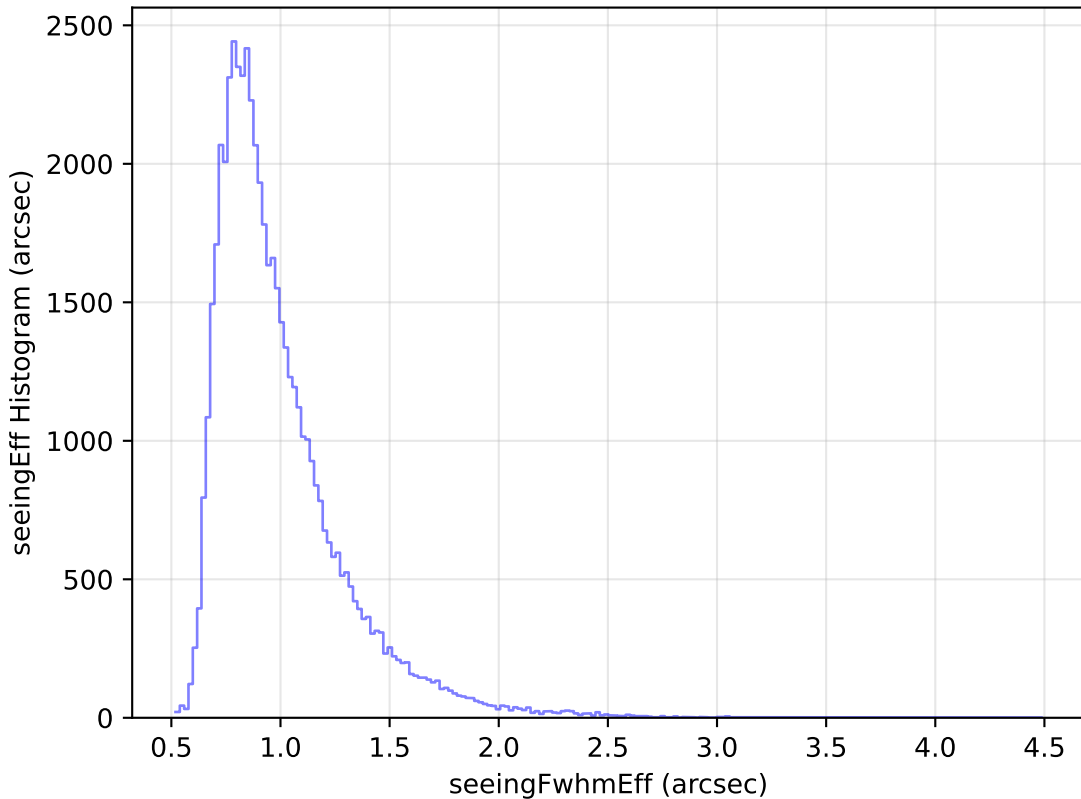
internal_u_expt30_nscale0.9v3.4_10yrs Yr 1 i band: seeingEff Histogram
