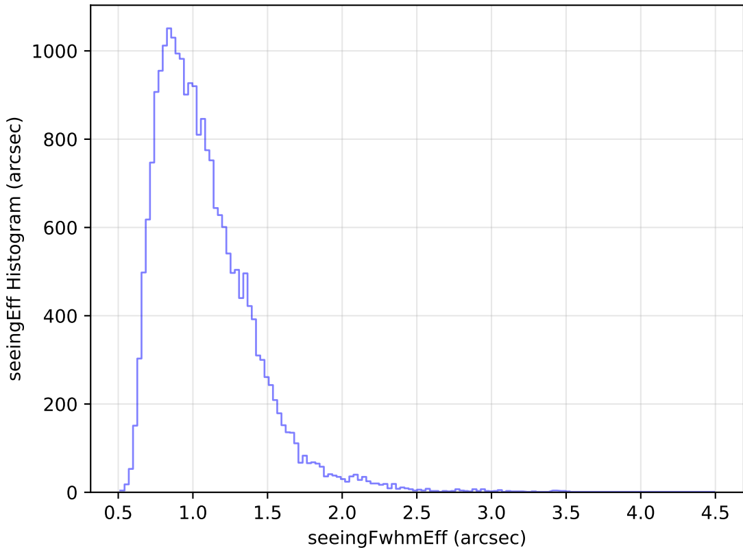
internal_u_expt30_nscale0.9v3.4_10yrs Yr 1 g band: seeingEff Histogram
