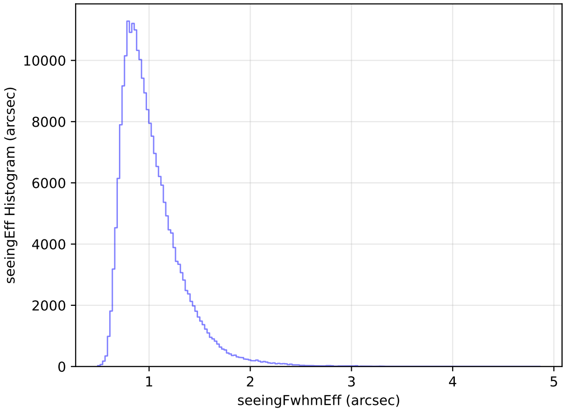
internal_u_expt30_nscale0.9v3.4_10yrs Yr 1 all bands: seeingEff Histogram
