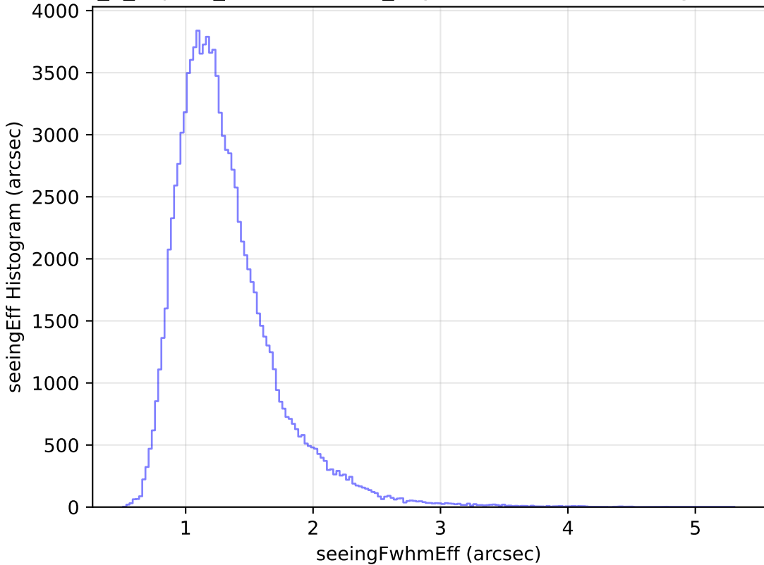
internal_u_expt30_nscale0.9v3.4_10yrs WFD u band: seeingEff Histogram
