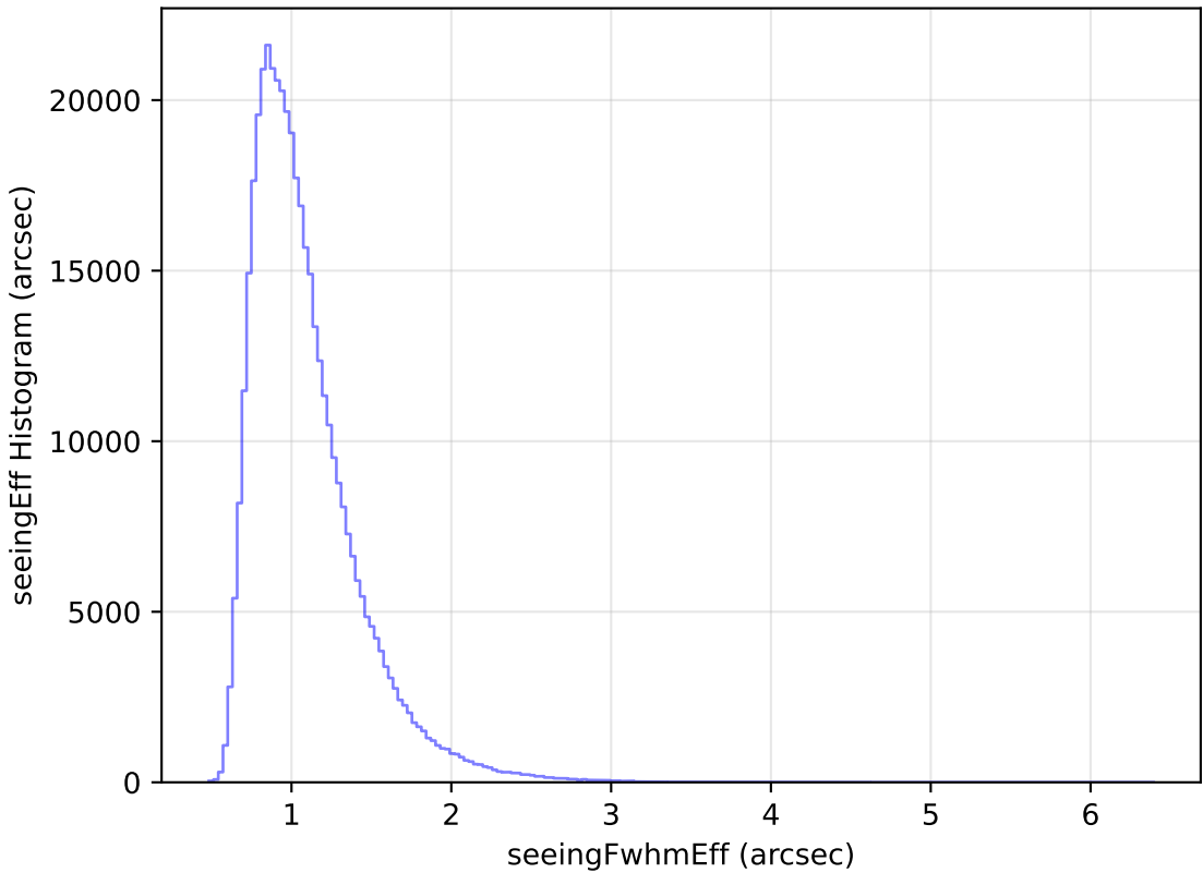
internal_u_expt30_nscale0.9v3.4_10yrs All sky z band: seeingEff Histogram
