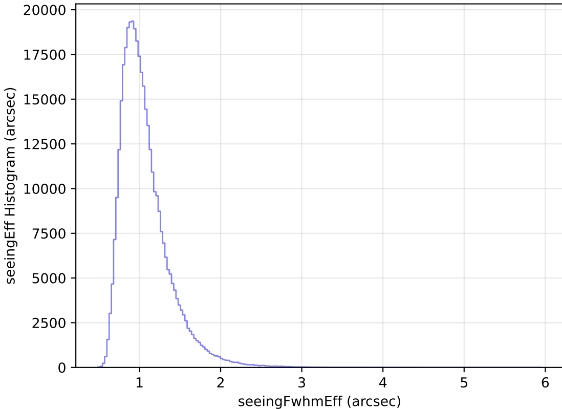
internal_u_expt30_nscale0.9v3.4_10yrs All sky y band: seeingEff Histogram
