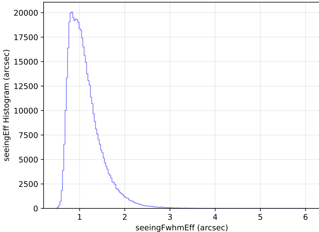
internal_u_expt30_nscale0.9v3.4_10yrs All sky r band: seeingEff Histogram
