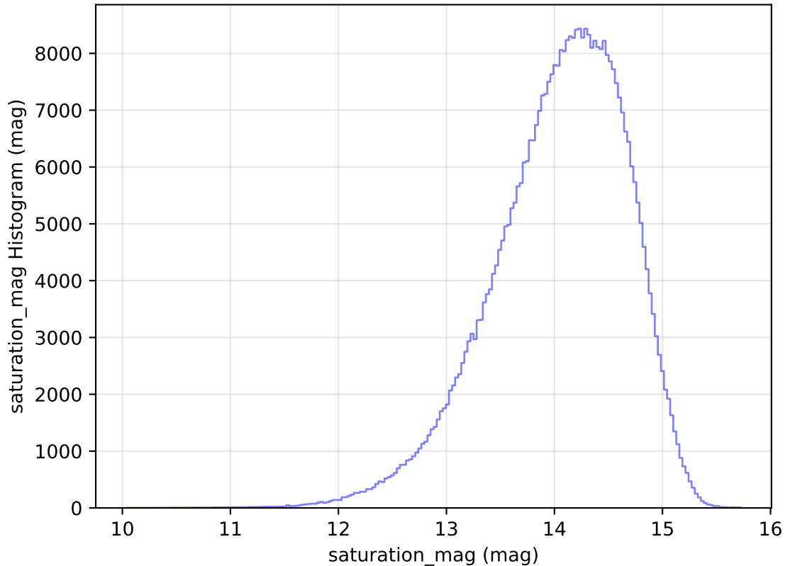
internal_u_expt30_nscale0.9v3.4_10yrs WFD z band: saturation_mag Histogram
