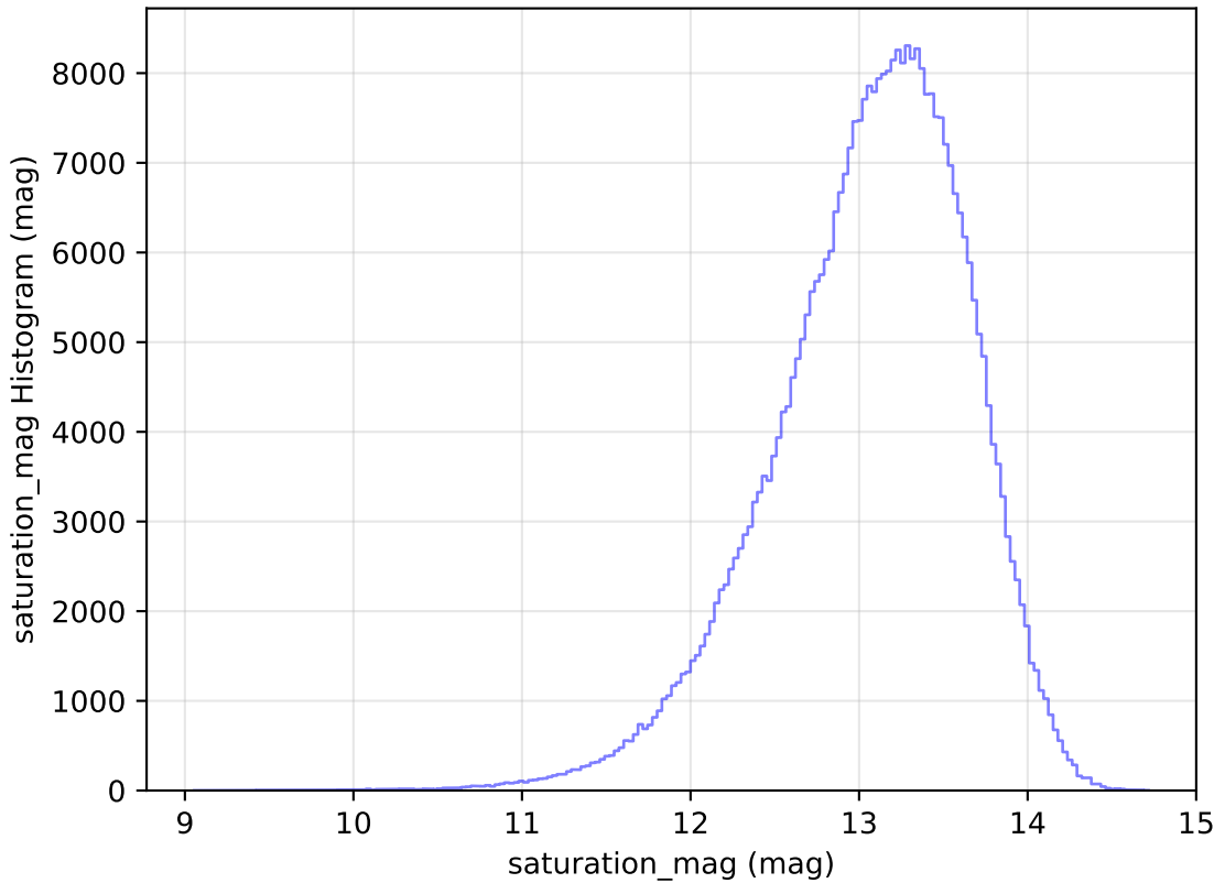
internal_u_expt30_nscale0.9v3.4_10yrs WFD y band: saturation_mag Histogram
