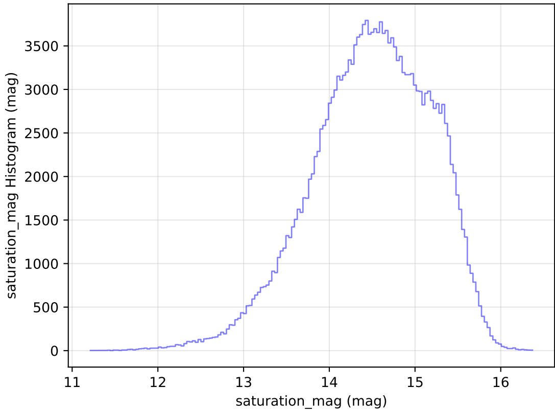
internal_u_expt30_nscale0.9v3.4_10yrs WFD g band: saturation_mag Histogram
