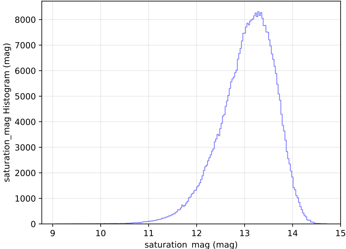
internal_u_expt30_nscale0.9v3.4_10yrs All sky y band: saturation_mag Histogram
