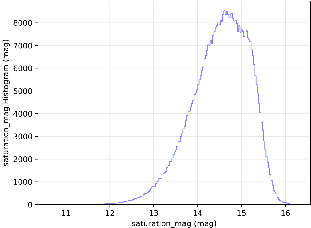
internal_u_expt30_nscale0.9v3.4_10yrs All sky r band: saturation_mag Histogram
