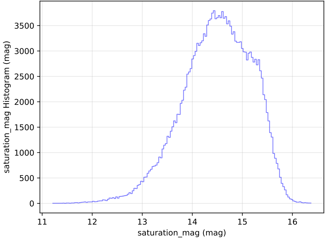
internal_u_expt30_nscale0.9v3.4_10yrs All sky g band: saturation_mag Histogram
