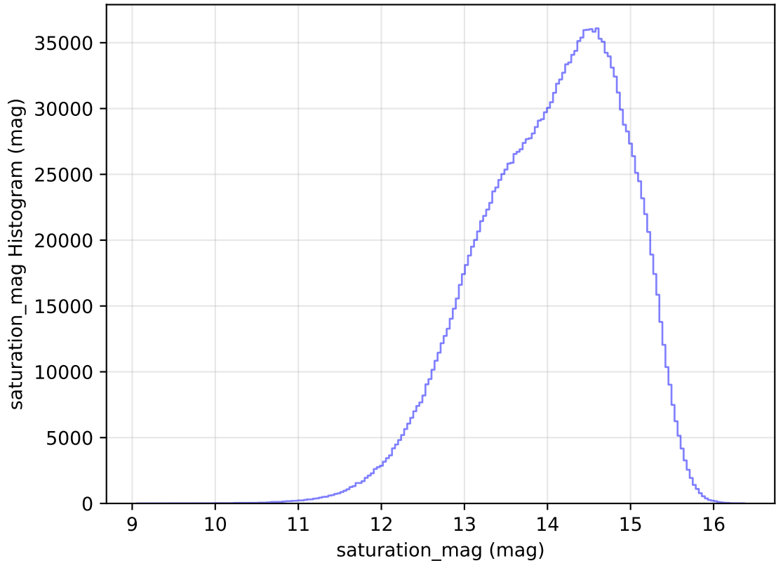
internal_u_expt30_nscale0.9v3.4_10yrs All sky all bands: saturation_mag Histogram
