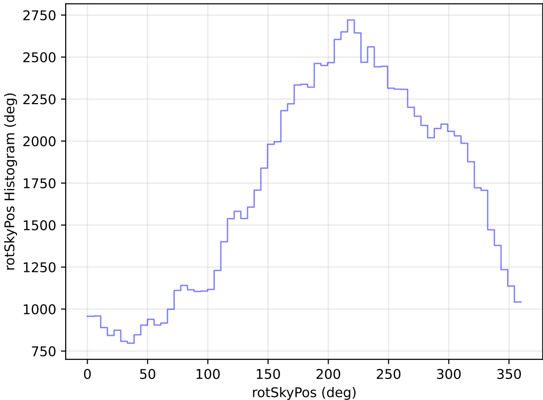
internal_u_expt30_nscale0.9v3.4_10yrs WFD u band: rotSkyPos Histogram
