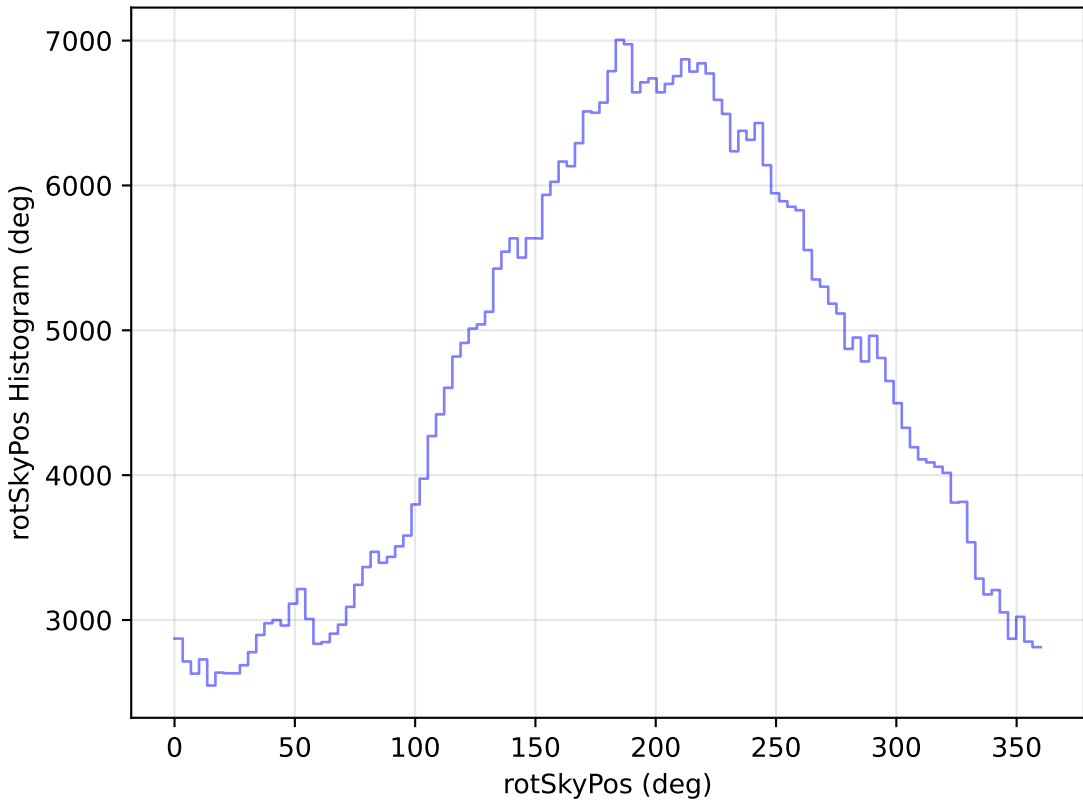
internal_u_expt30_nscale0.9v3.4_10yrs WFD r band: rotSkyPos Histogram
