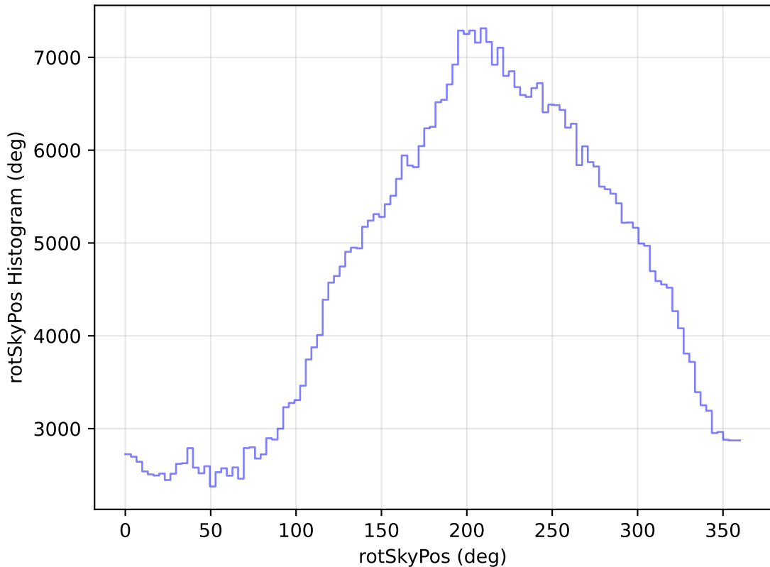
internal_u_expt30_nscale0.9v3.4_10yrs WFD i band: rotSkyPos Histogram
