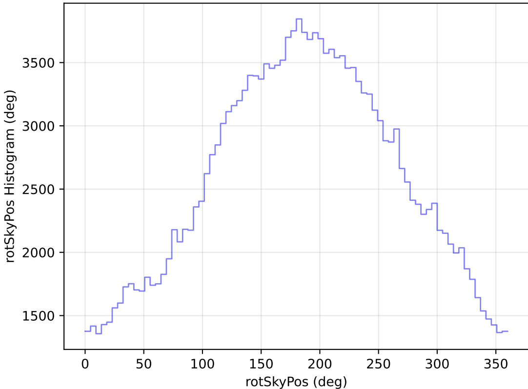
internal_u_expt30_nscale0.9v3.4_10yrs WFD g band: rotSkyPos Histogram
