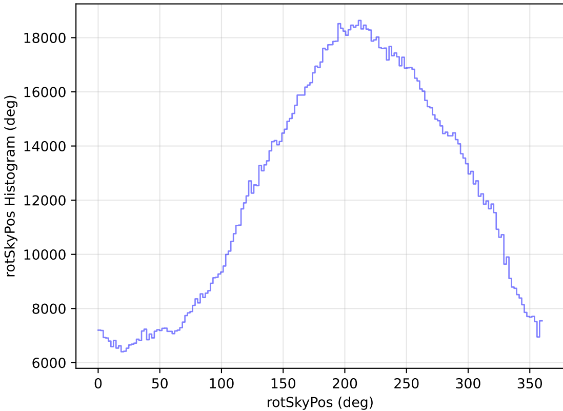
internal_u_expt30_nscale0.9v3.4_10yrs WFD all bands: rotSkyPos Histogram
