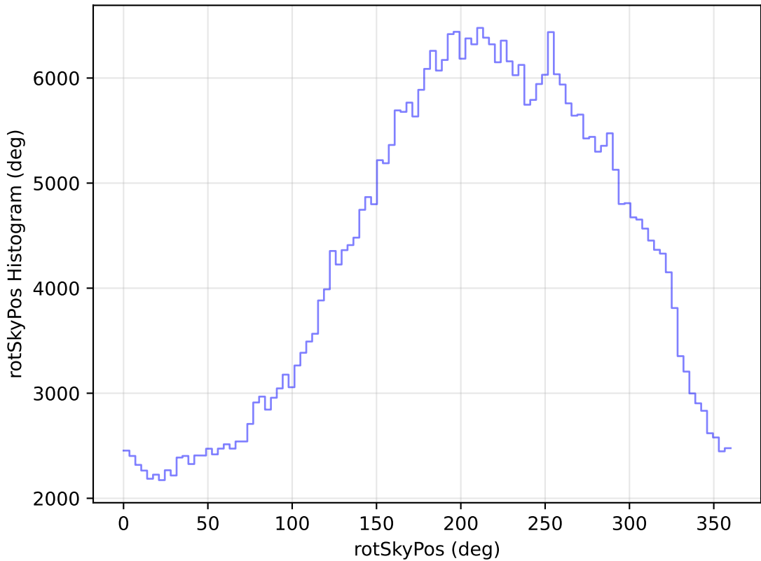
internal_u_expt30_nscale0.9v3.4_10yrs All sky z band: rotSkyPos Histogram
