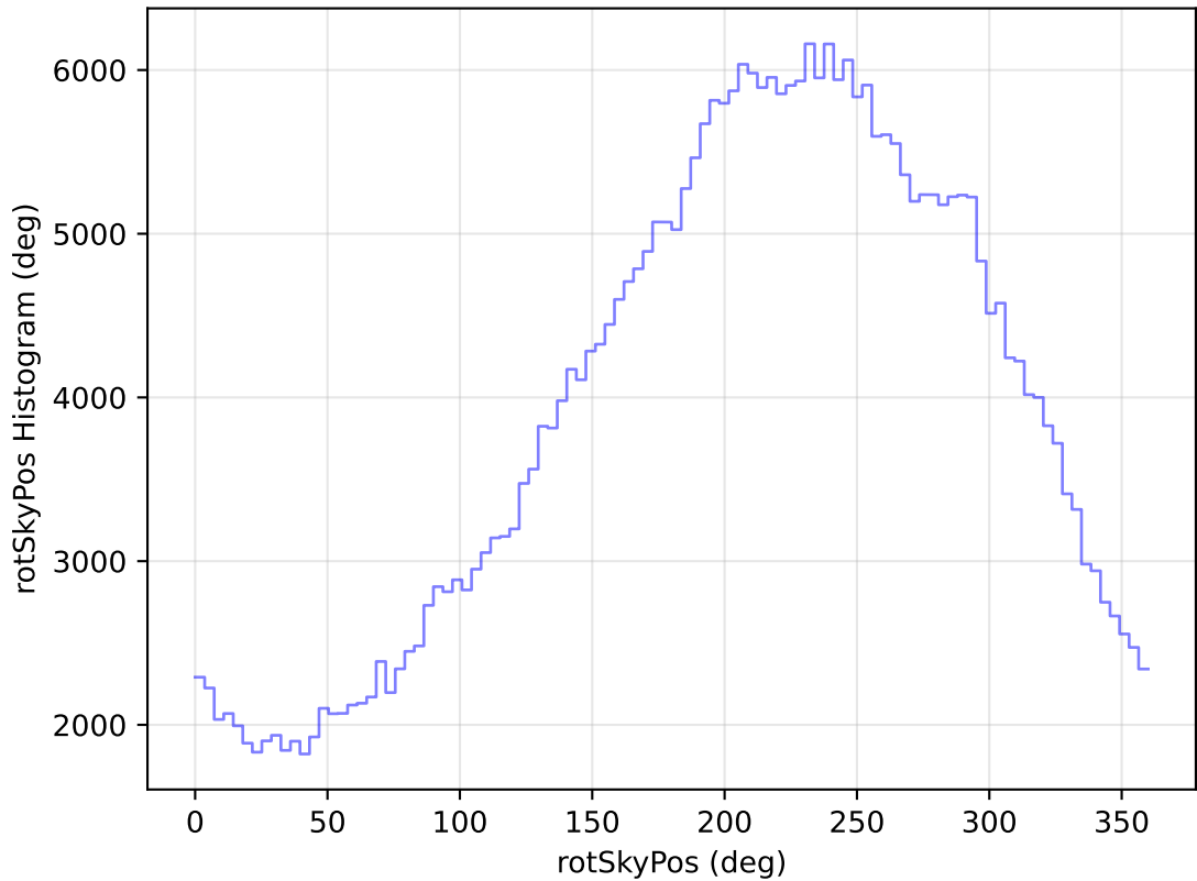
internal_u_expt30_nscale0.9v3.4_10yrs All sky y band: rotSkyPos Histogram
