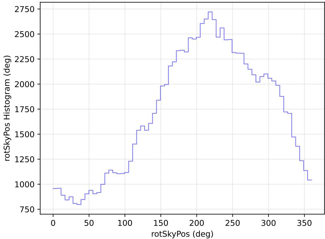
internal_u_expt30_nscale0.9v3.4_10yrs All sky u band: rotSkyPos Histogram
