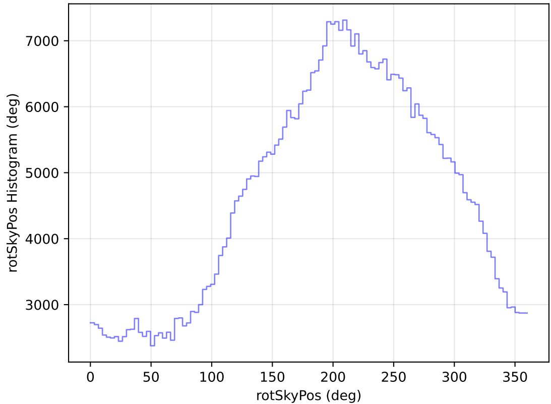
internal_u_expt30_nscale0.9v3.4_10yrs All sky i band: rotSkyPos Histogram
