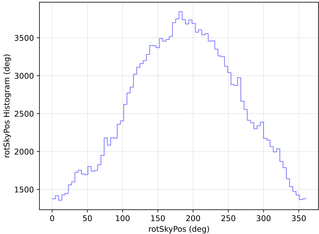
internal_u_expt30_nscale0.9v3.4_10yrs All sky g band: rotSkyPos Histogram
