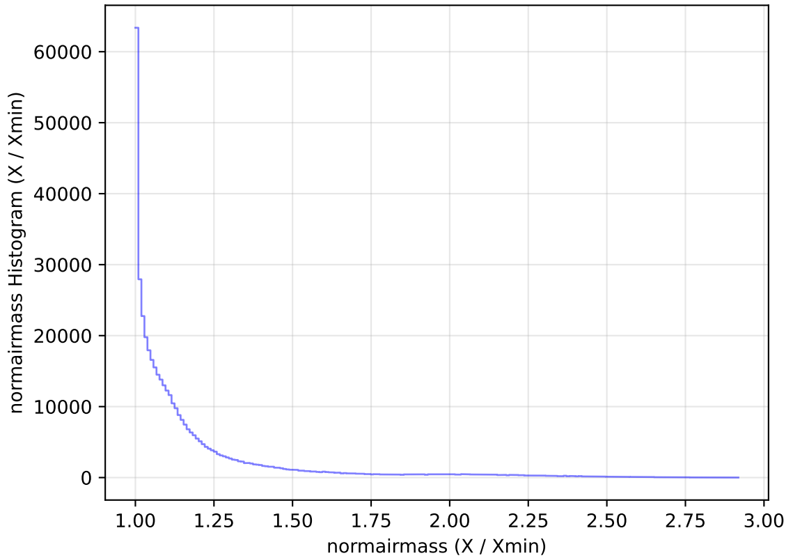
internal_u_expt30_nscale0.9v3.4_10yrs WFD z band: normairmass Histogram
