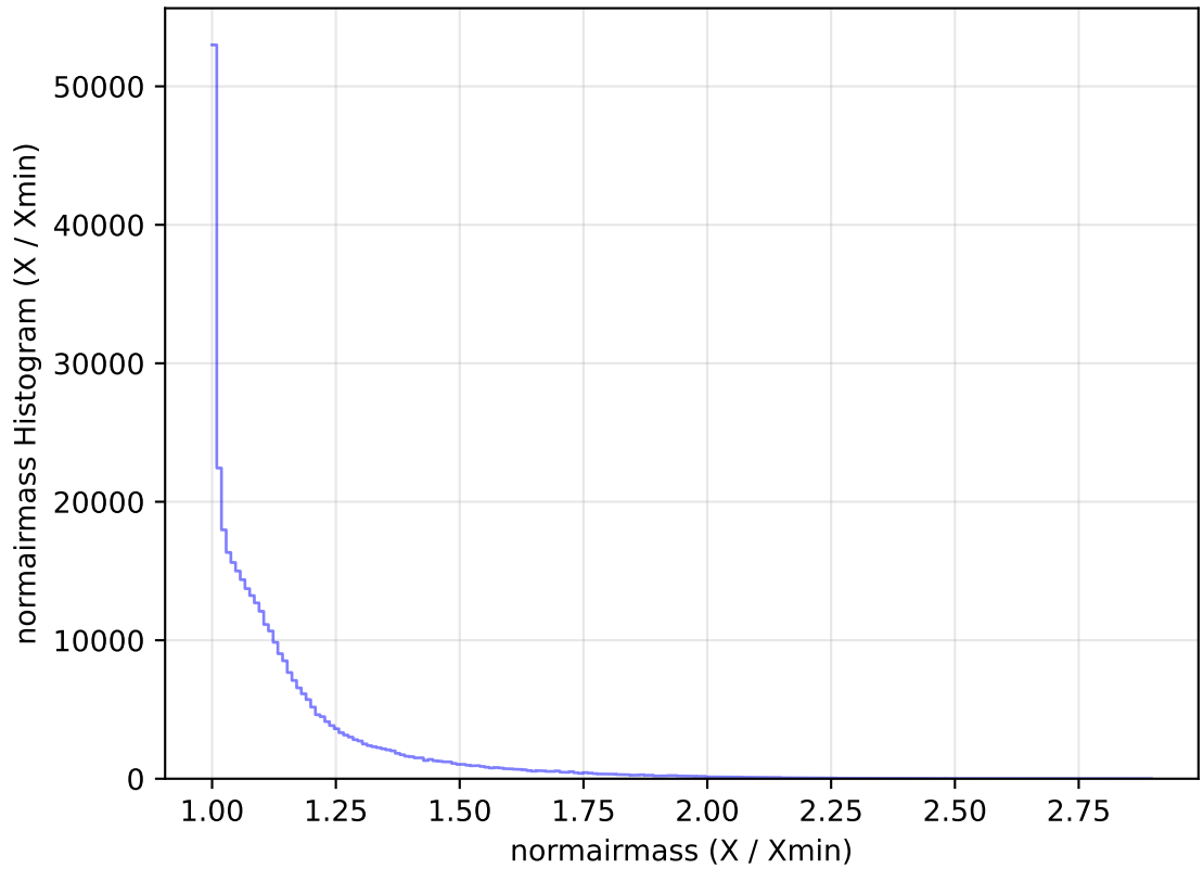
internal_u_expt30_nscale0.9v3.4_10yrs WFD y band: normairmass Histogram
