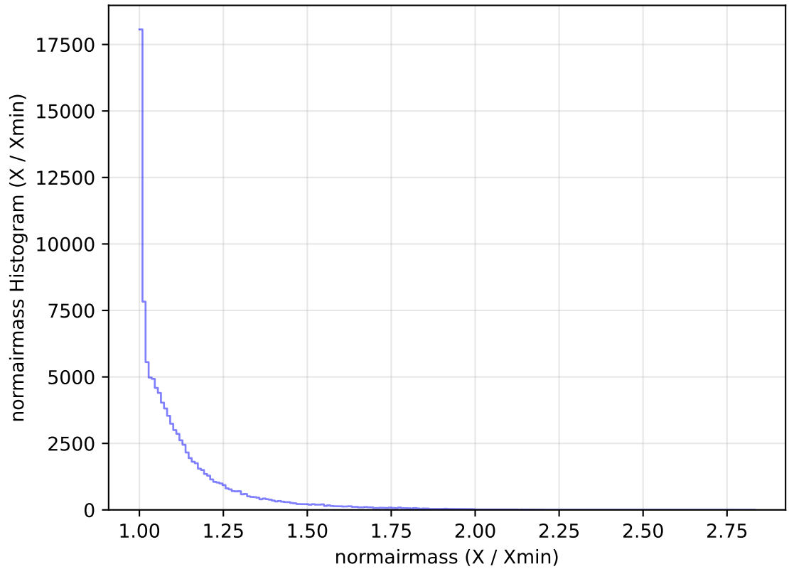
internal_u_expt30_nscale0.9v3.4_10yrs WFD u band: normairmass Histogram
