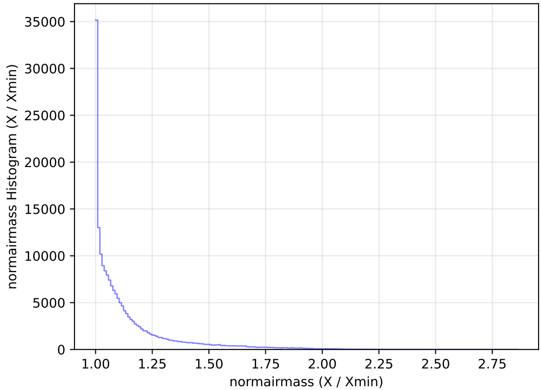
internal_u_expt30_nscale0.9v3.4_10yrs WFD g band: normairmass Histogram
