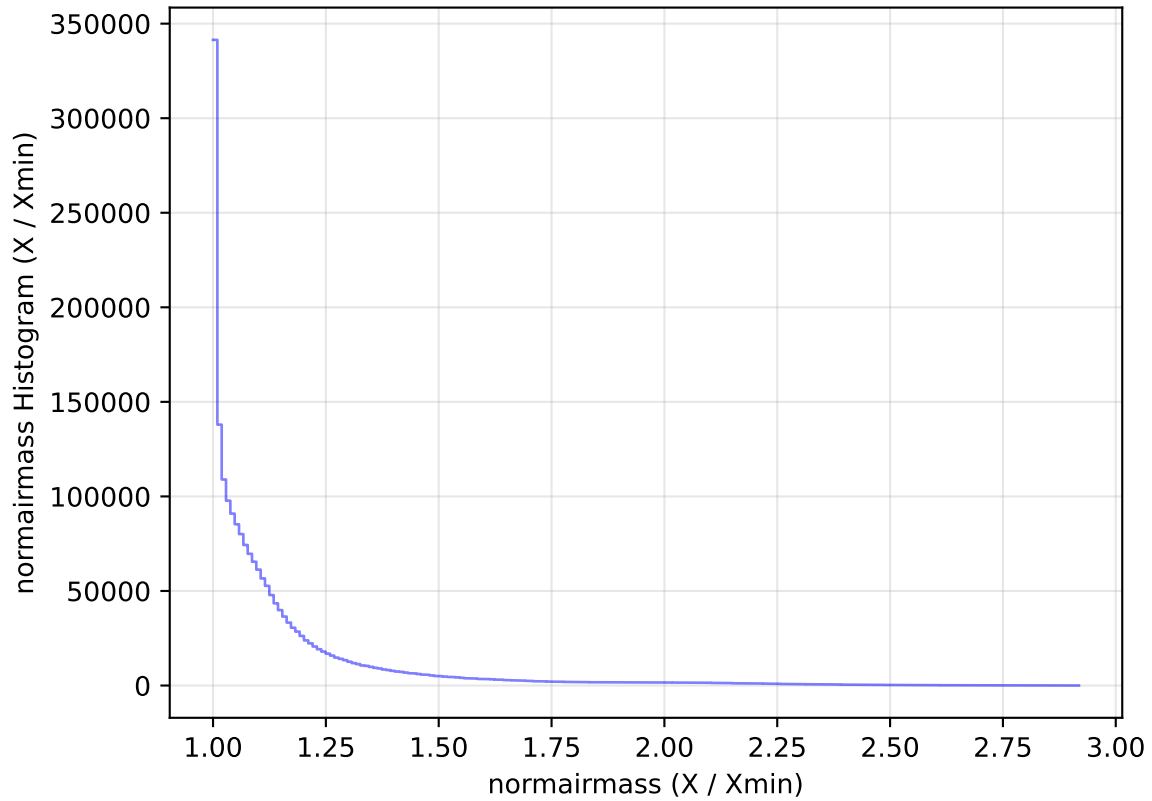
internal_u_expt30_nscale0.9v3.4_10yrs WFD all bands: normairmass Histogram
