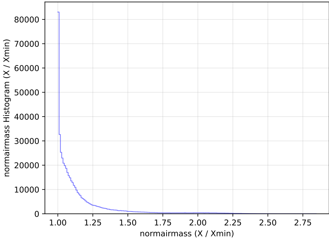
internal_u_expt30_nscale0.9v3.4_10yrs All sky r band: normairmass Histogram
