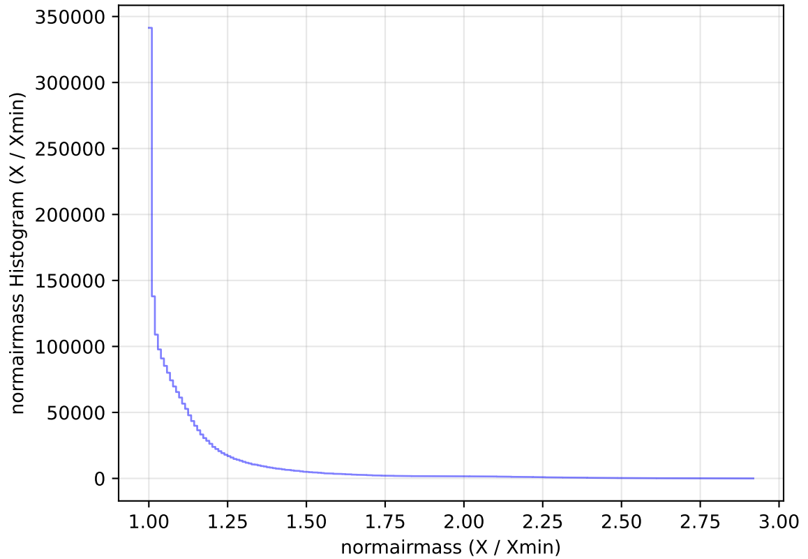
internal_u_expt30_nscale0.9v3.4_10yrs All sky all bands: normairmass Histogram
