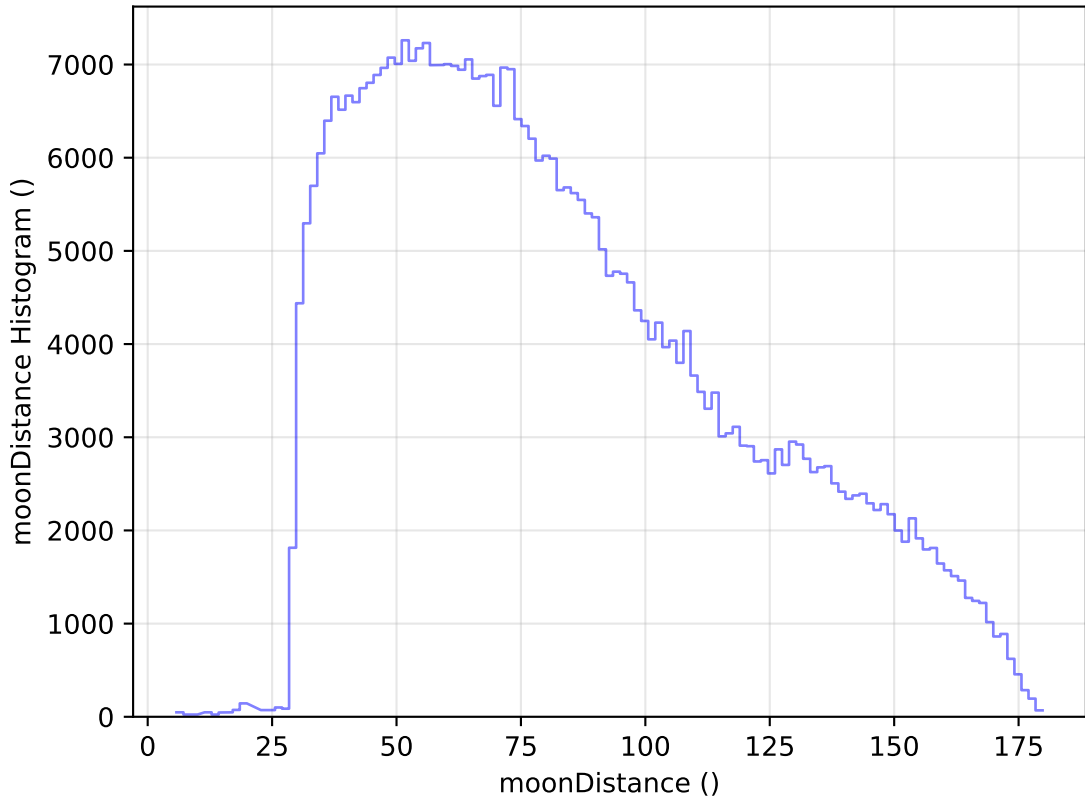
internal_u_expt30_nscale0.9v3.4_10yrs WFD z band: moonDistance Histogram
