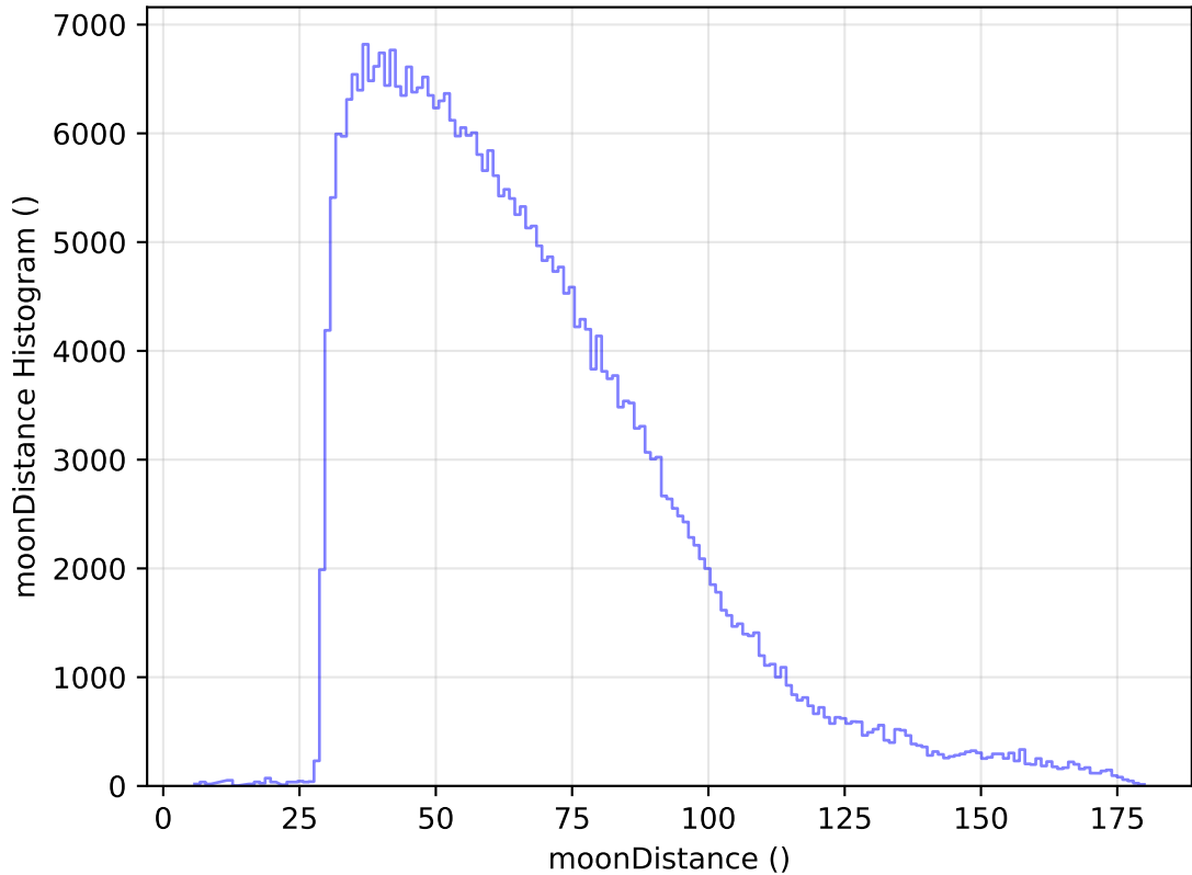
internal_u_expt30_nscale0.9v3.4_10yrs WFD y band: moonDistance Histogram
