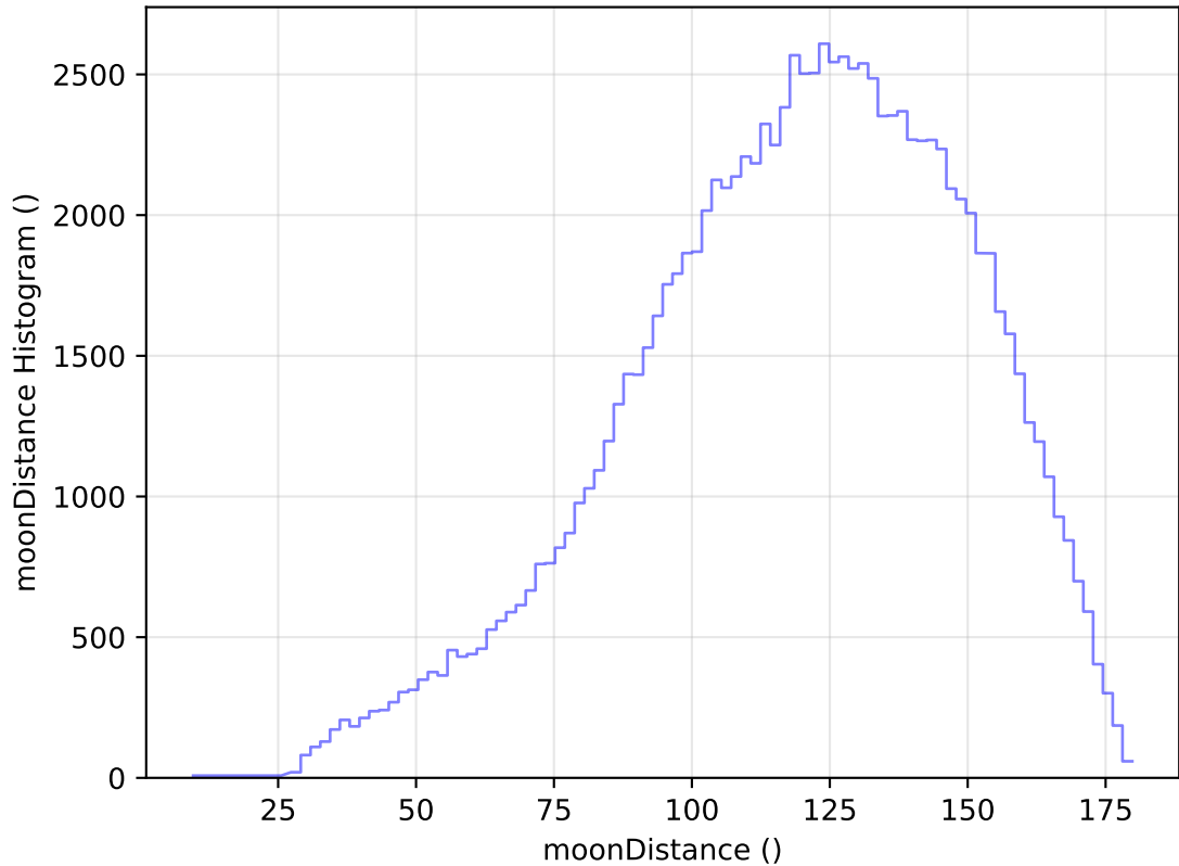
internal_u_expt30_nscale0.9v3.4_10yrs WFD u band: moonDistance Histogram
