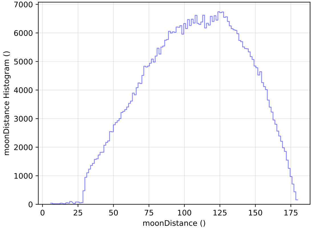
internal_u_expt30_nscale0.9v3.4_10yrs WFD r band: moonDistance Histogram
