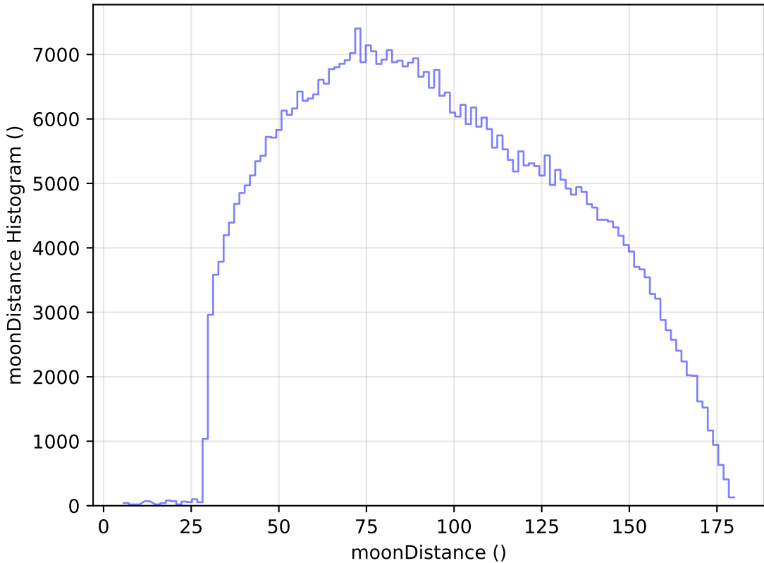
internal_u_expt30_nscale0.9v3.4_10yrs WFD i band: moonDistance Histogram
