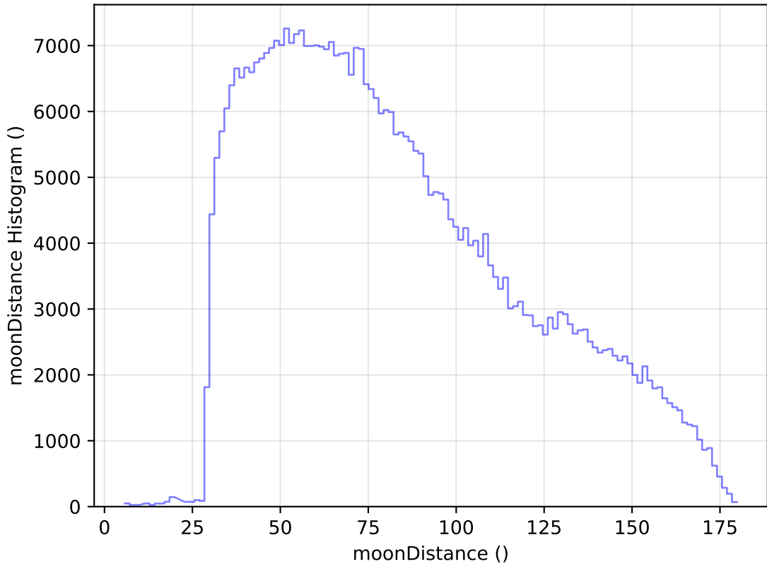
internal_u_expt30_nscale0.9v3.4_10yrs All sky z band: moonDistance Histogram
