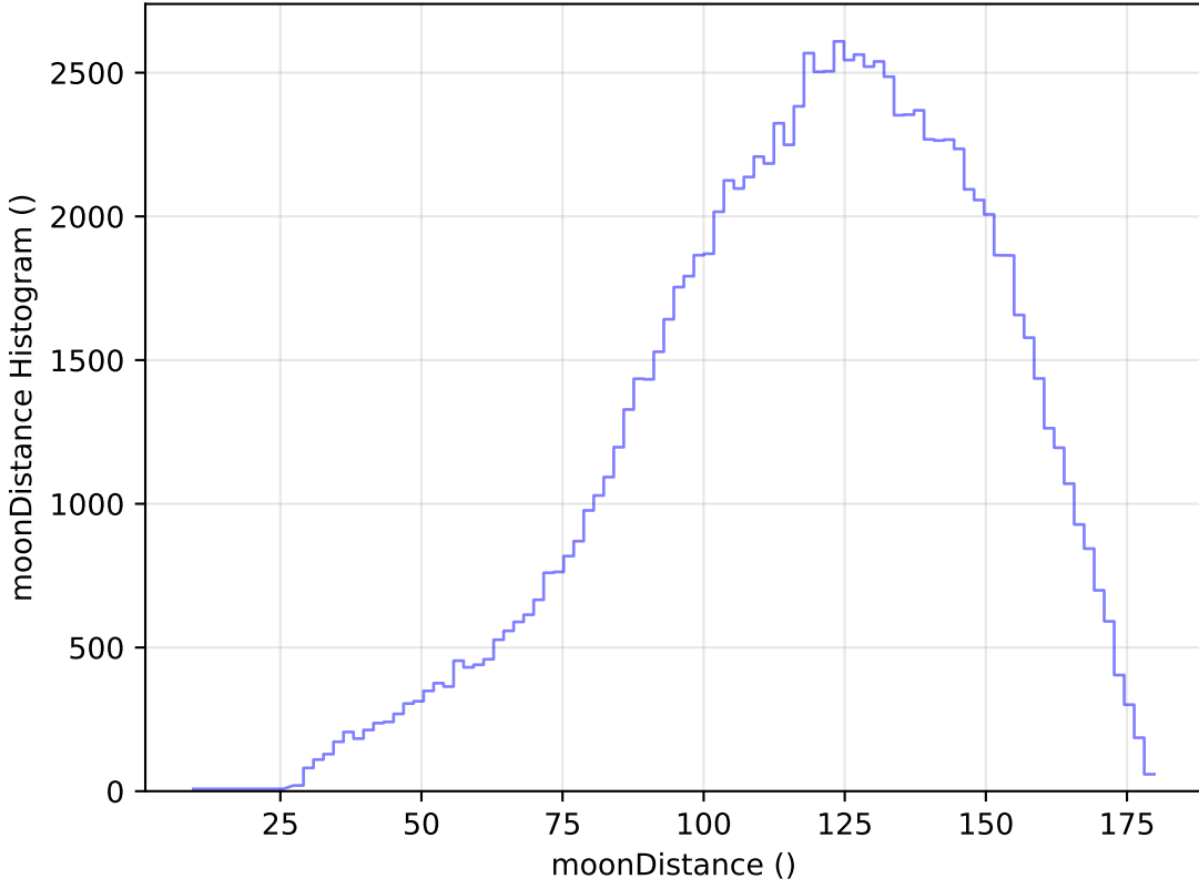
internal_u_expt30_nscale0.9v3.4_10yrs All sky u band: moonDistance Histogram
