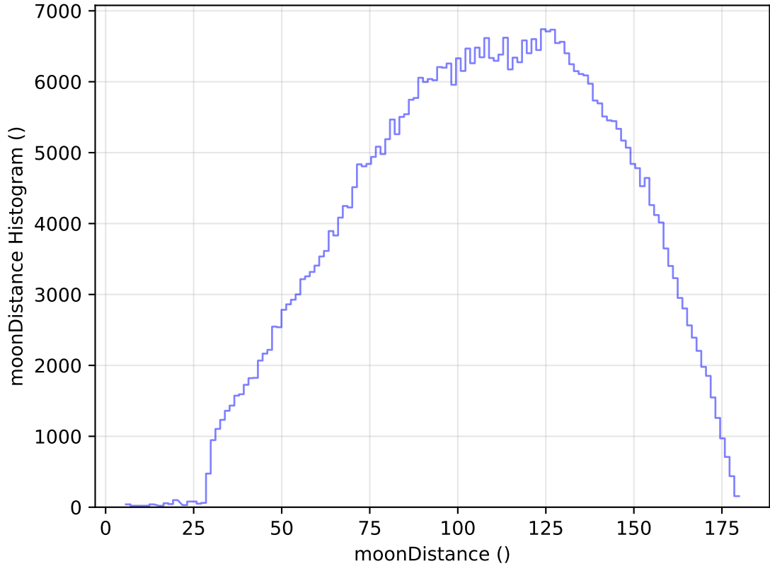
internal_u_expt30_nscale0.9v3.4_10yrs All sky r band: moonDistance Histogram
