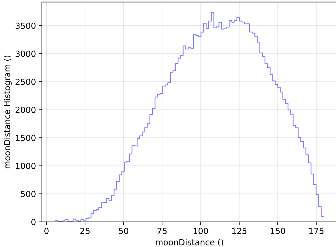
internal_u_expt30_nscale0.9v3.4_10yrs All sky g band: moonDistance Histogram
