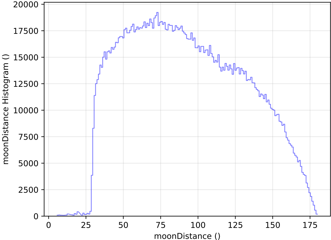
internal_u_expt30_nscale0.9v3.4_10yrs All sky all bands: moonDistance Histogram
