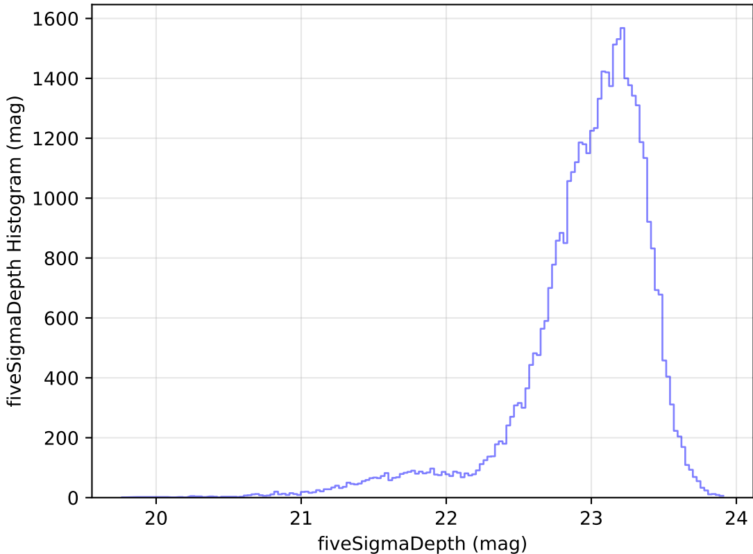
internal_u_expt30_nscale0.9v3.4_10yrs Yr 1 z band: fiveSigmaDepth Histogram
